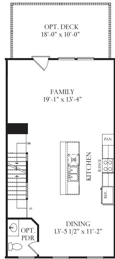
Second Floor Plan @ Mid-Kitchen
